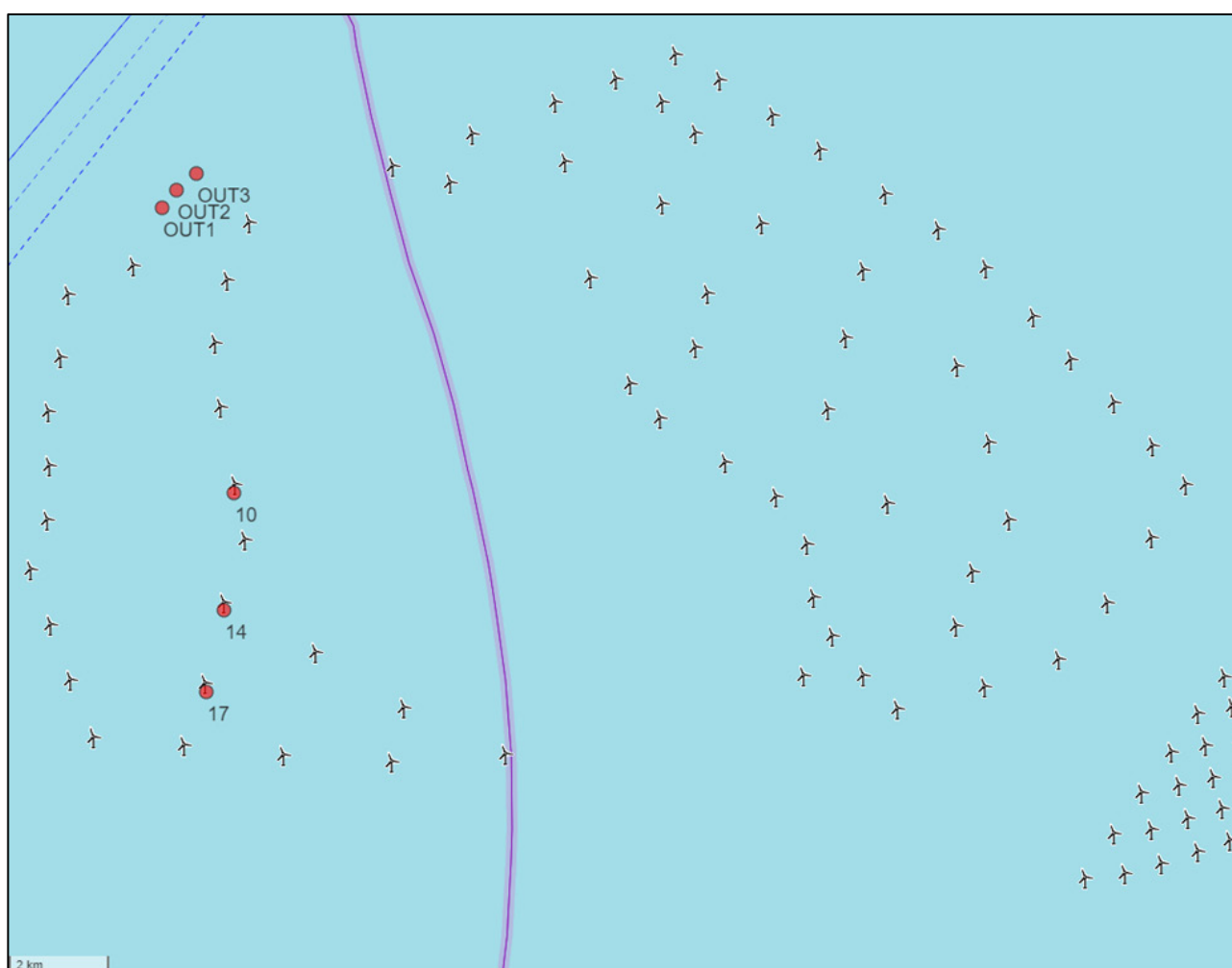
Figure 3.5. Map visualizing the distribution of wind turbines at Kriegers Flak and the sample station locations inside the windfarm (10, 14 and 17) and outside (OUT) the windfarm. Sample locations are marked with red dots.
