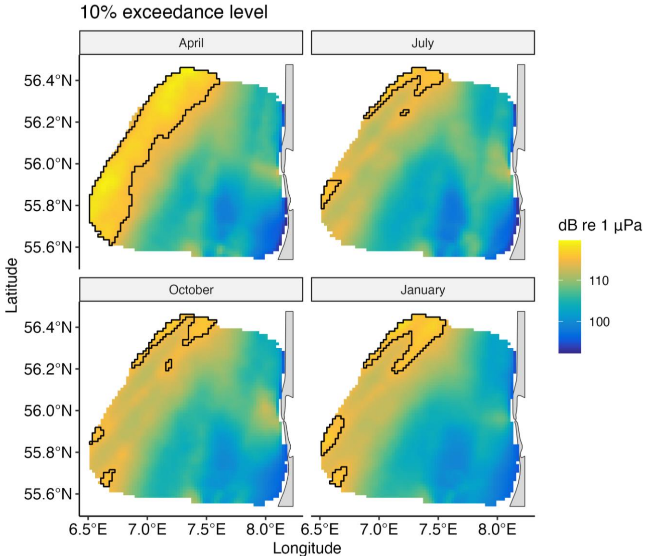
Figure 4-35 Maps of the 10% exceedance level in the 125Hz decidecade frequency band for April 2023, July 2023, October 2023 and January 2024 representing the four seasons. The sound pressure level ( L_{p,125\text{Hz } ddec} , unit dB re 1 \mu Pa/decidecade) measured on a short time scale of a few seconds (the temporal scale of the individual snap shots modelled every hour of the month) in each point of the map is expected to be equal to or higher than the level corresponding to the colour 5% of the time. The map therefore represents the loudest events that occur in the survey area for the four months. The overlaid black polygons represents parts of the map where sound pressure levels ( L_{p,125\text{Hz } ddec} ) exceed 115 dB re 1 \mu Pa (i.e., the noise level above which harbour porpoises are expected to respond) 10% of the time, indicating that reactions to the noise is expected to occur on average 10% of the time.
