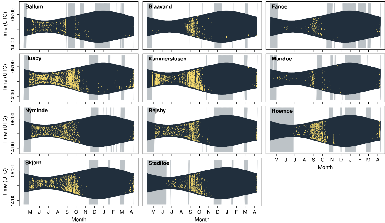
Figure 4.12. Nightly activity overview for Nathusis' pipistrelle across all onshore locations. Dates (x-axis) range over one year, from April 10, 2023, to April 10, 2024. Time (y-axis) ranges from noon on a given day until noon the next day. Data points are activity minutes. Each point represents a minute with at least five call detections within a 3-5 second window (see section 3.3.2). Black background: nighttime from solar sunset to solar sunrise. Grey background: days without active deployments.
